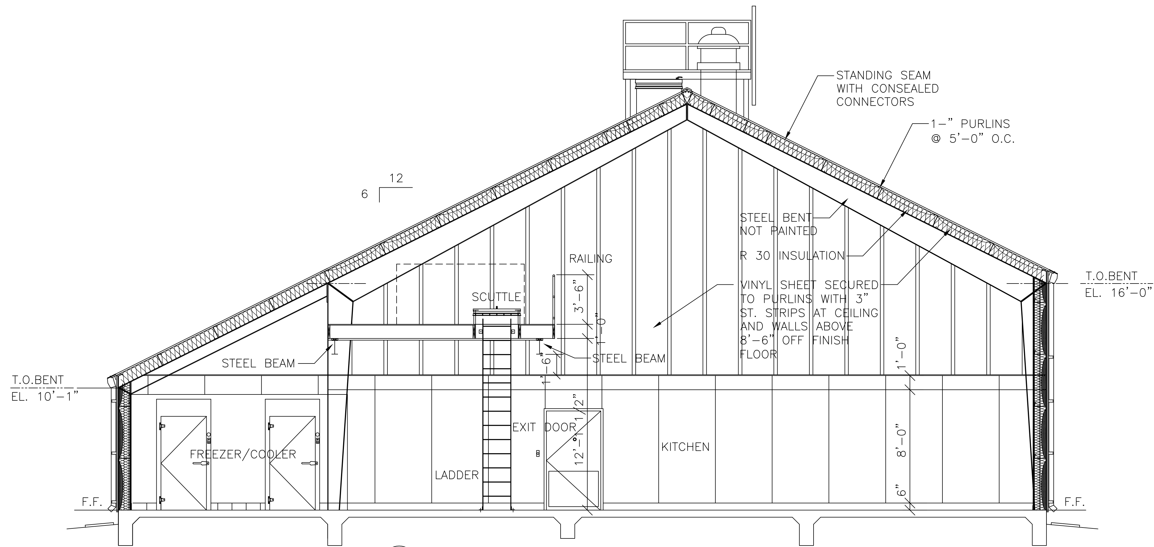
1 BUILDING SECTION A4.1 SCALE: 1/4"=1'-0"
