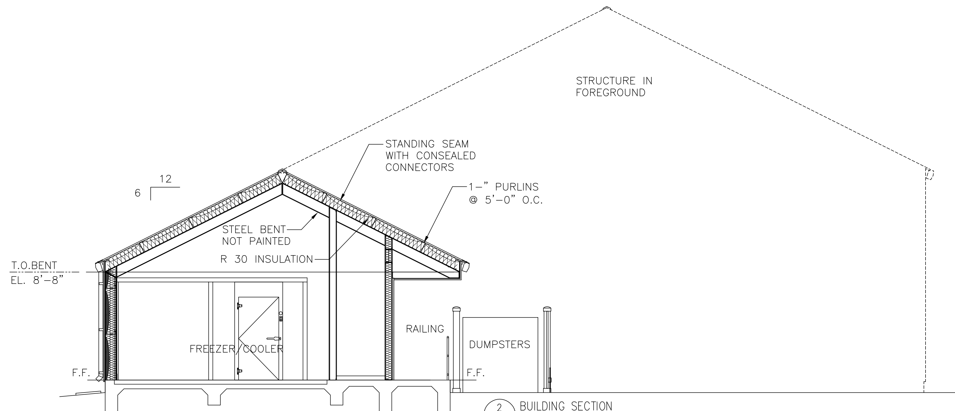
2 BUILDING SECTION A4.1 SCALE: 1/4"=1'-0"
