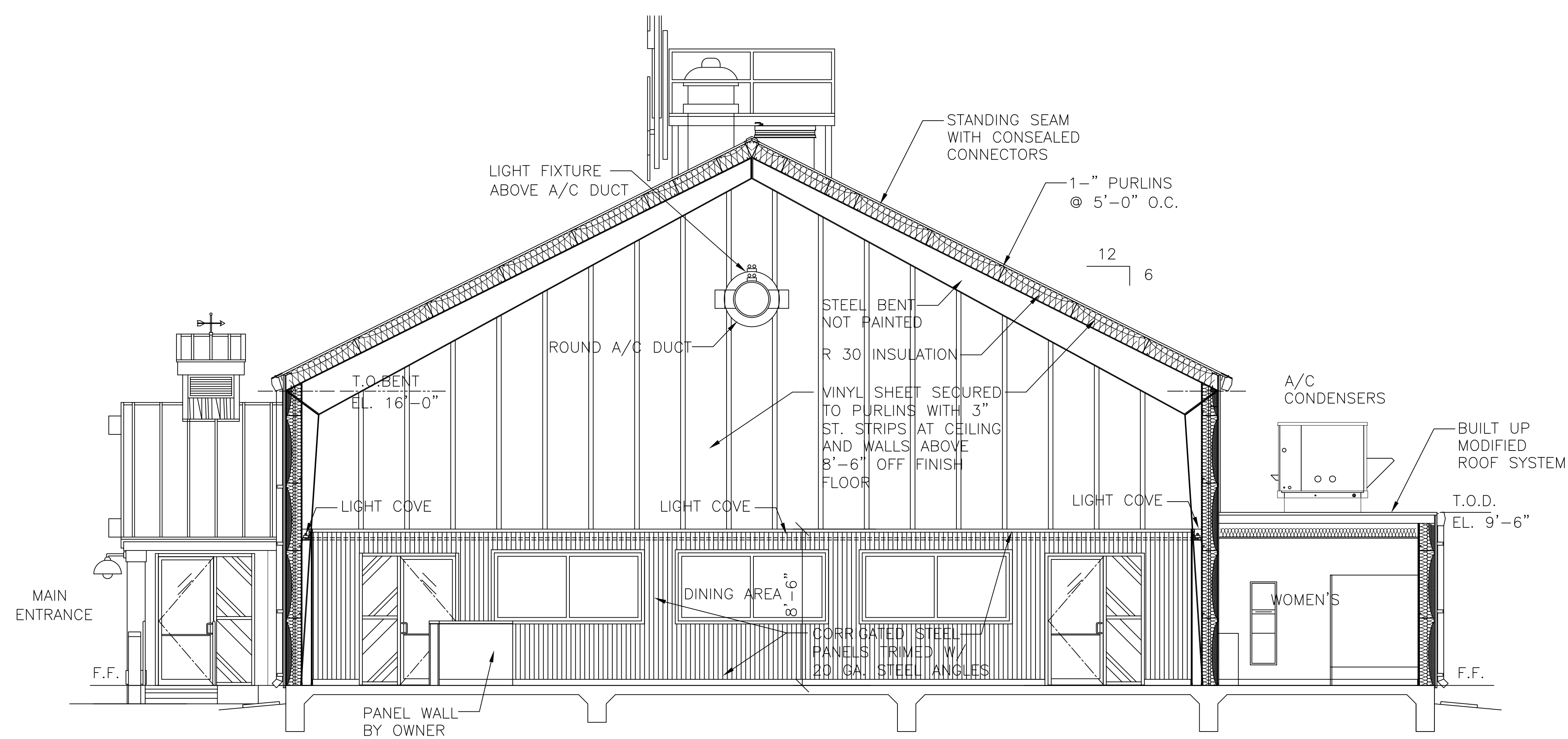
1 BUILDING SECTION A4.0R SCALE: 1/4"=1'-0"
